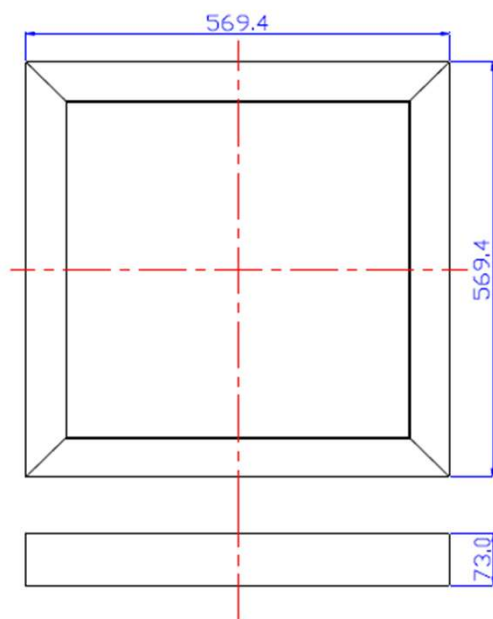
Dimensions of SOL
