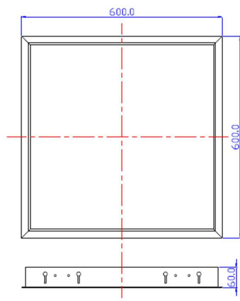
Dimensions of holding frame
