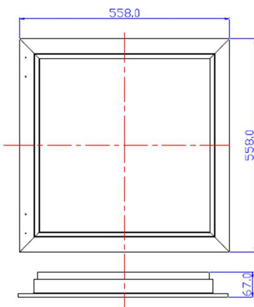
Dimensions of SOL
