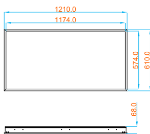
Holding Frame: 1210*610*68mm
