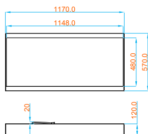
SOL: 1170*570*120mm
