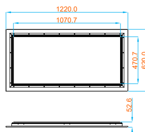
Front Frame: 1220*620*52.6mm
